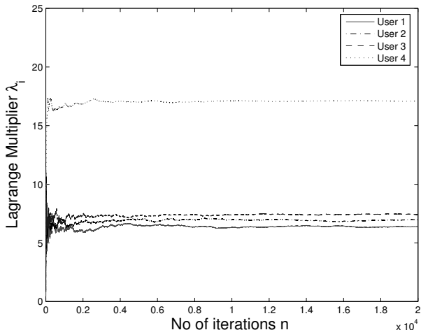
Fig. 2. Convergence for Markovian channel model
