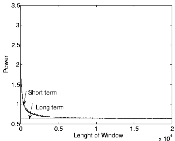
Fig. 4. Power required for the short term fairness compared to long term fairness
