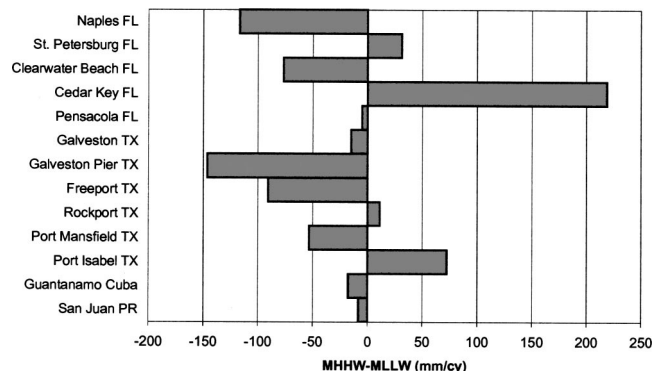
Fig. 2. Gulf Coast diurnal tide range trends
