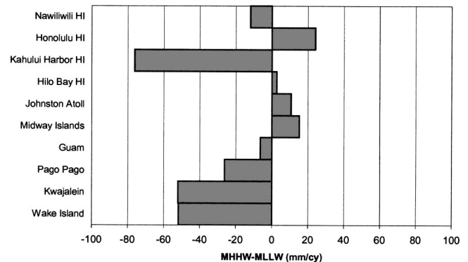
Fig. 6. Pacific Islands diurnal tide range trends
