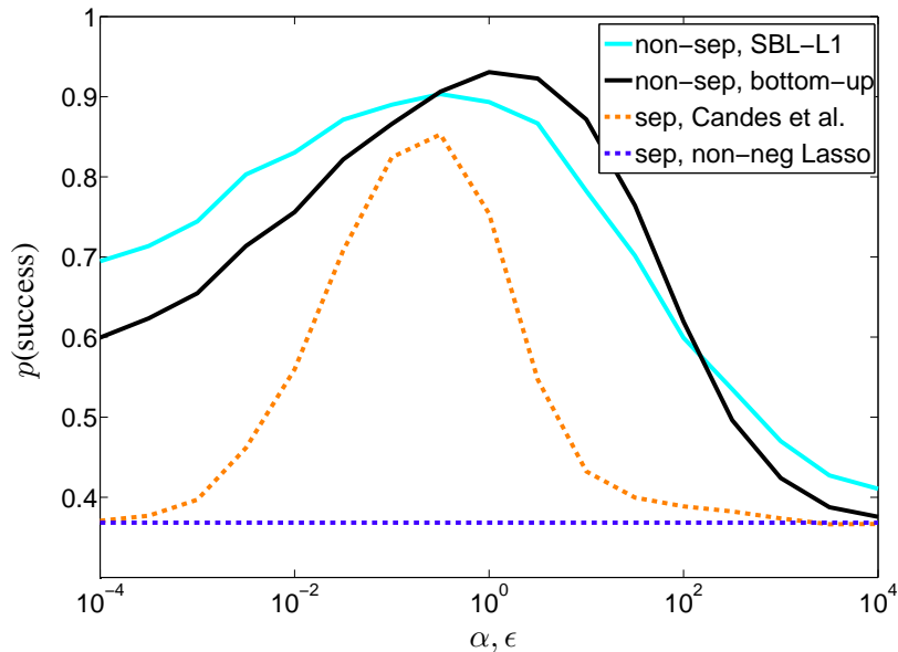
Fig. 4. Probability of success recovering sparse, non-negative coefficients as a function of \alpha, \epsilon using 10 reweighted \ell_1 iterations. The non-negative Lasso has no such parameter, so its performance is flat.
