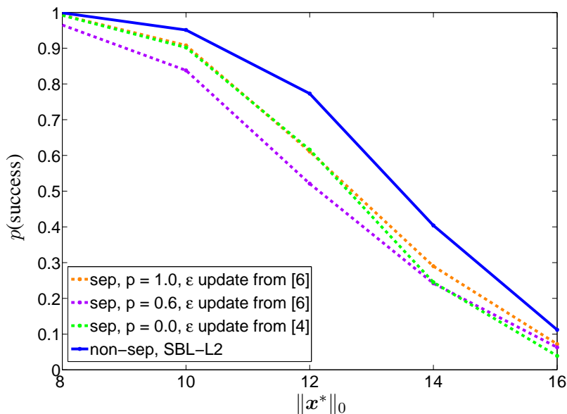
Fig. 1. Iterative reweighted \ell_2 example using unit magnitude nonzero coefficients. Probability of success recovering sparse coefficients for different sparsity values, i.e., \|\mathbf{x}^*\|_0 .
