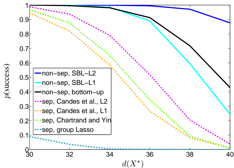
Fig. 5. Iterative reweighted results using 5 simultaneous signal vectors. Probability of success recovering sparse coefficients for different row sparsity values, i.e., d(X^*) .
