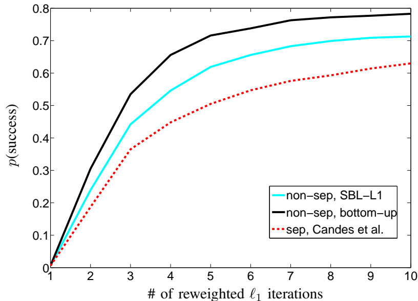
Fig. 3. Non-negative sparse coding example. Probability of success recovering sparse, non-negative coefficients as the number of reweighted \ell_1 iterations is increased.
